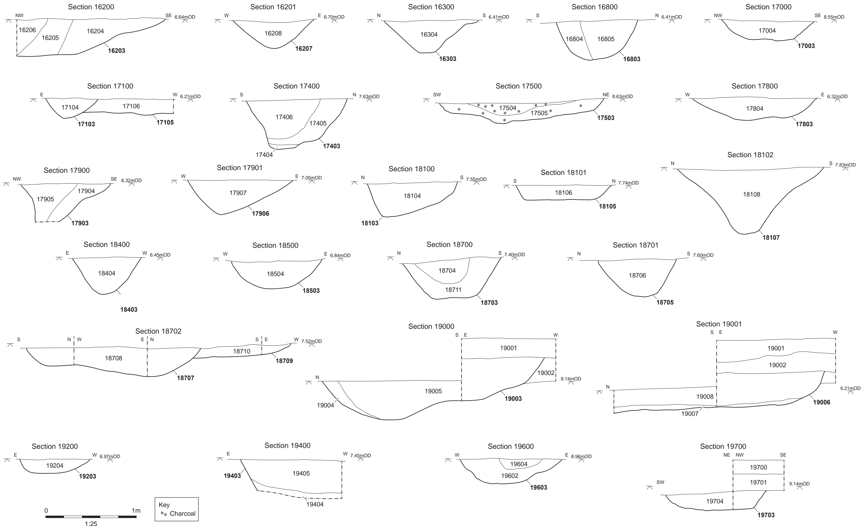
Figure 20: Sections (Trenches 162-3, 168, 170-1, 174-5, 178-9, 181, 184-5, 187, 190, 192, 194 and 196-7)
